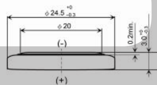
Dimension Drawing
