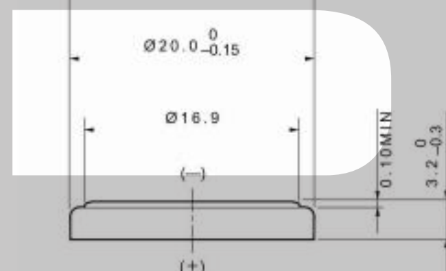
Dimension Drawing
